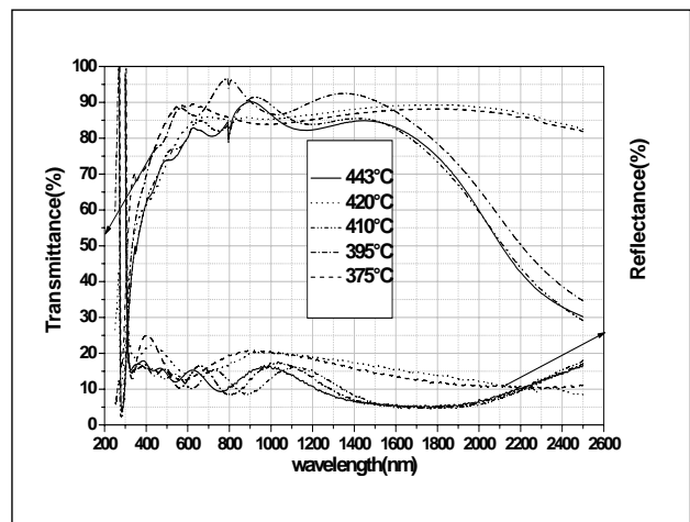
Fig. 3 Transmittance and reflectance spectra of SnO 2 films deposited at different temperatures on glass substrate
