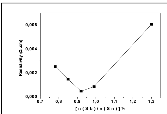
Fig. 4 Transmittance, reflectance a) and resistivity b) upon [\text{n}(\text{Sb})/\text{n}(\text{Sn})] % concentration respectively, ( T_s=443^\circ\text{C} , \text{O}_2 : 2 L/min) showing that the best resistivity correspond to the weakest reflectance
