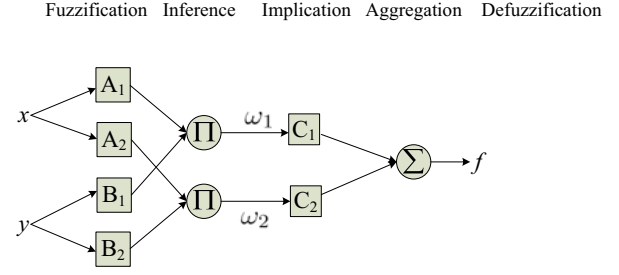
Fig. 3. General model of Mamdani ANFIS
