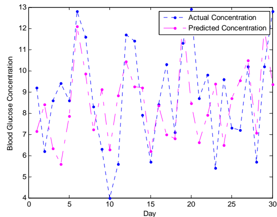
Fig. 4. An enlarged segment of the time-series in Fig. 3, for the first 30 days
