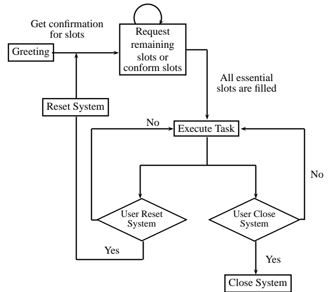
Fig. 3. The dialogue strategy learned by LA learning algorithm
