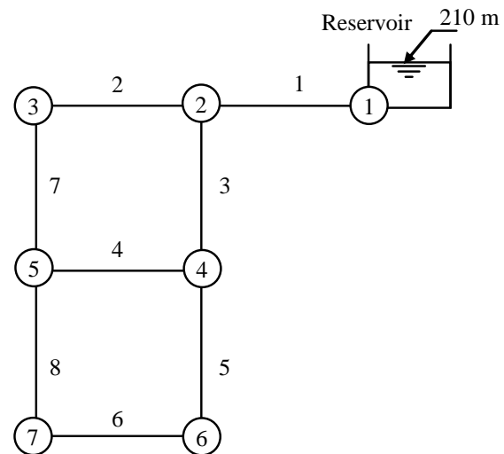
Fig. 3 Two-Loop Network
