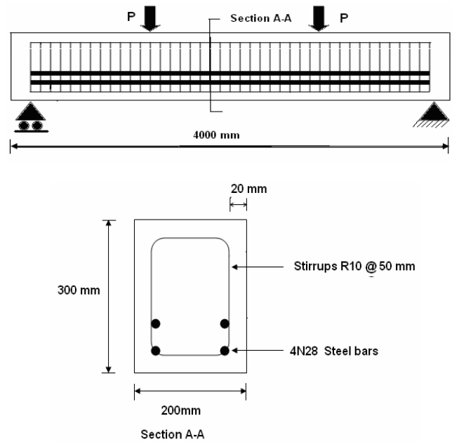
Fig. 2 Reference beam details
