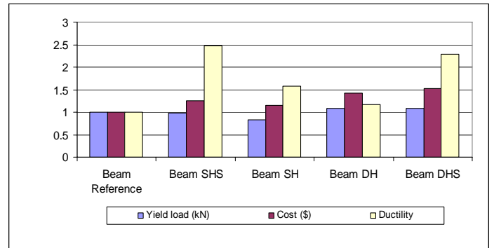
Fig. 7 Beam cost VS Ductility and strength
