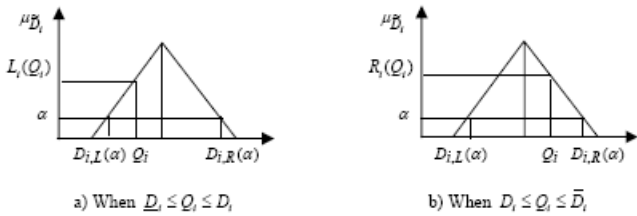
Fig. 1 Alpha cut of \tilde{D}_i
