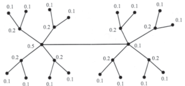
Fig.2 Fuzzy graph G
