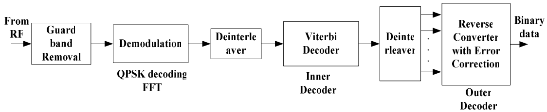
Fig. 8 Block diagram of receiver section
