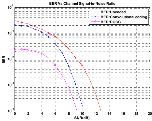
Fig. 9 BER versus SNR for uncoded, convolutional coded and RCCC OFDM system
