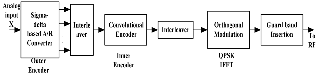
Fig. 6 Block diagram of transmitter section
