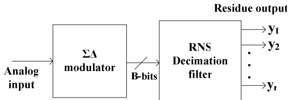
Fig. 2 Sigma-delta based parallel A/R converter
