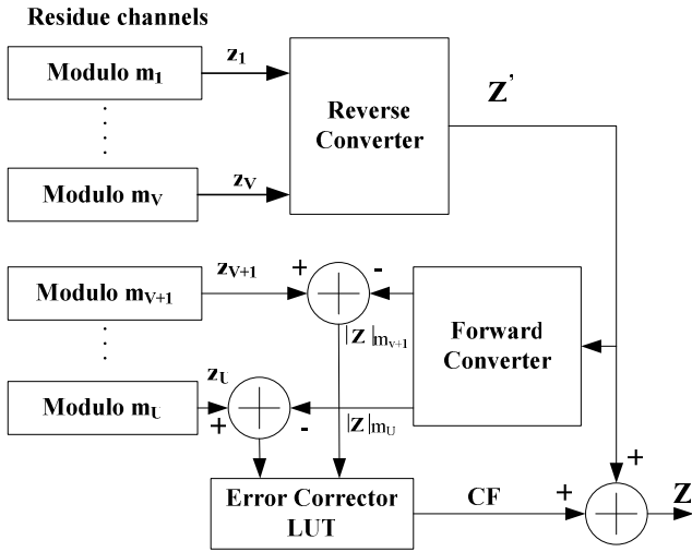
Fig. 1 Principle of error correction with RRNS
