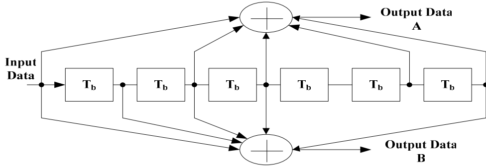
Fig. 7 Convolutional encoder
