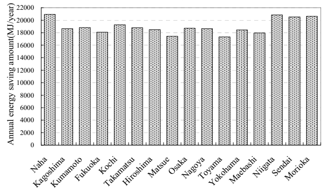
Fig. 8 Annual energy saving amount
