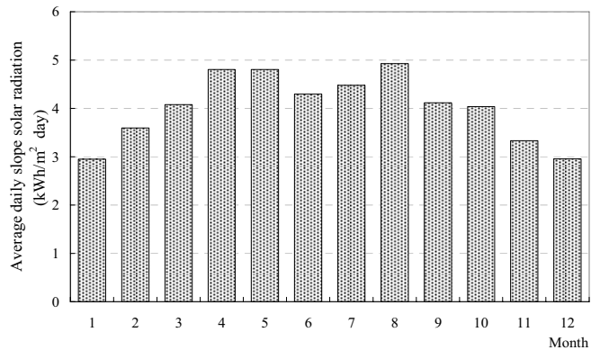
Fig. 4 Whole country average daily slope solar radiation amount
