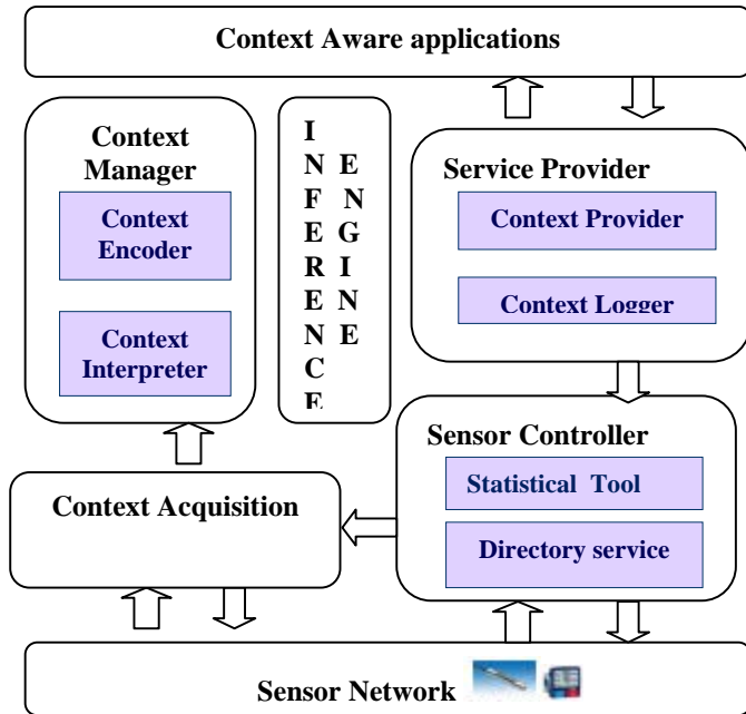
Fig. 1 CALEEF Architecture
