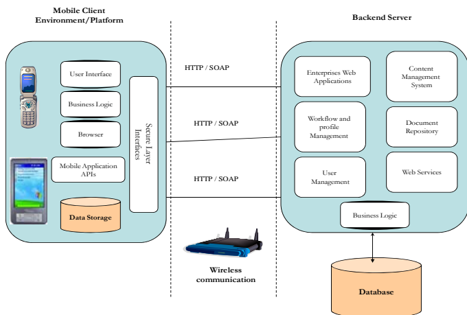
Fig. 1 Mobile Applications Development Framework
