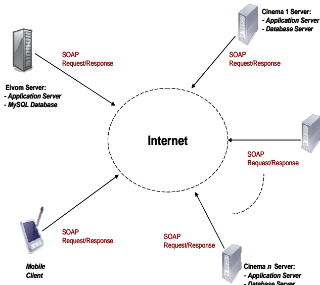
Fig. 2 Mobile Movie System
