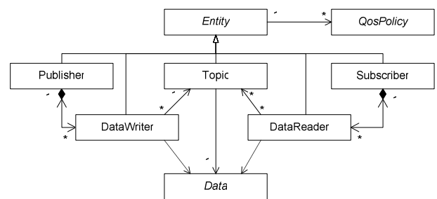
Fig. 2 Simplified Class diagram of the DCPS model (adopted from [10])
