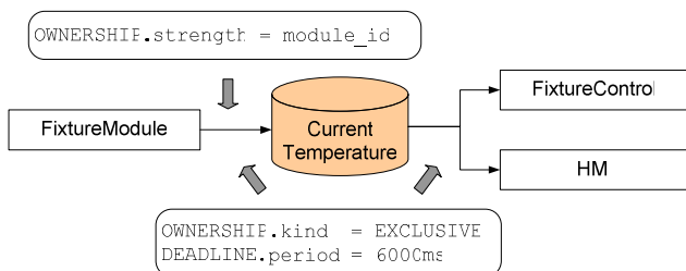
Fig. 8 QoS settings for requirement III
