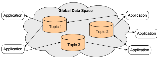
Fig. 1 Overview of the publish/subscribe concept
