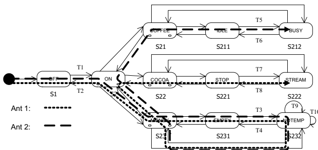
Figure 3 Optimal Solution
