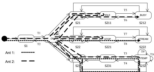
Figure 4 Solution Candidate
