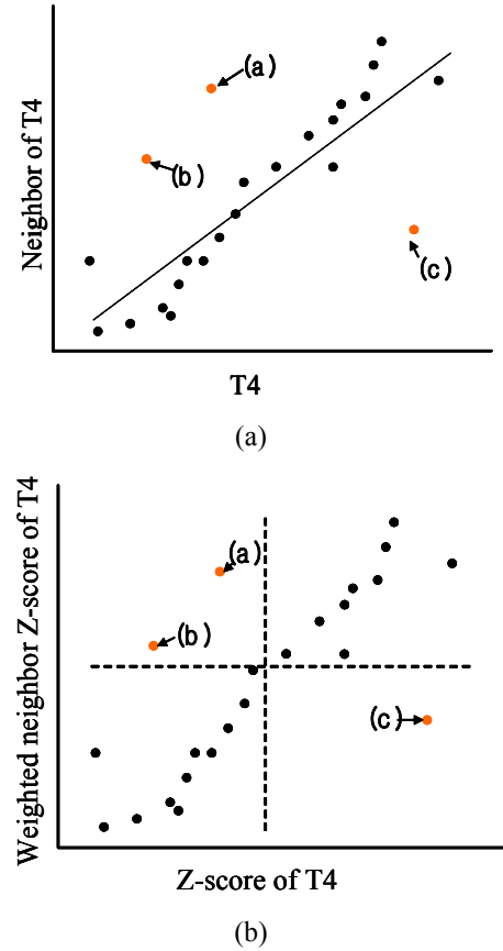
Fig. 1 Ordinary scatter plot(a) and Moran's scatter plot(b)
