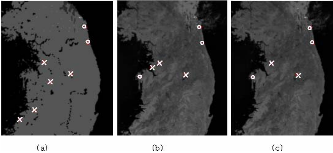
Fig. 4 Detection results using ordinary scatter plot(a), Moran's scatter plot(b), MODIS fire product(c)
