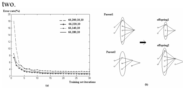
Figure 1 (a) Error rates on the test set of the MFNN versus 30 iterations through 60,000 MNIST pattern training set with fixed topologies. For example the name 66,220,10 indicates 66 input units, 10 output units and 220 hidden units. (b) Example of crossover applied on two MFNN individuals with different number of layers.
