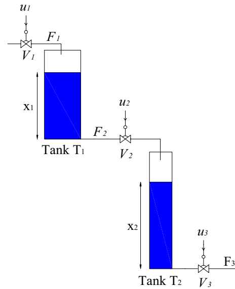
Fig. 1 Two-tank system
