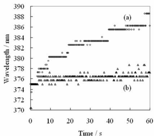
Fig. 5 Potential dependence of the peak position at around 380 nm obtained from time-resolved SOWG analysis synchronized with potential step measurements from -200 to -600 mV for 60 s in 0.3 \text{ mol dm}^{-3} KBr aqueous solutions containing 5 (a) and 1.25 \times 10^{-5} \text{ mol dm}^{-3} HV.
