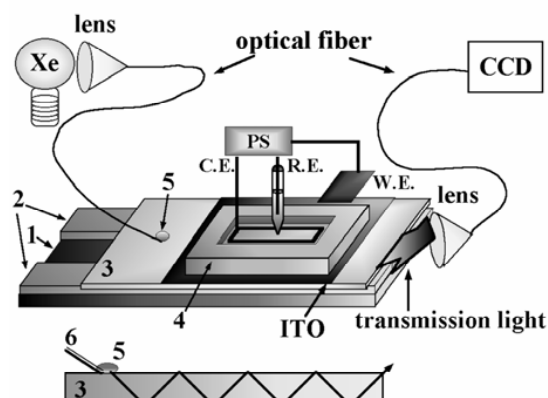
Fig. 1 Illustration of ITO-SOWG systems. 1: slide glass base, 2: silicon rubber strip acting SOWG supports, 3: SOWG (50 \times 20 \times 0.05 mm), 4: leak-proof silicone rubber solution cell, 5: glycerol drop, and 6: optical fiber from the light source. PS: Potentiostat, W.E., C.E., and R.E.: working (ITO), counter (Pt wire), and reference (Ag/AgCl) electrode, and ITO: indium-tin-oxide electrode.
