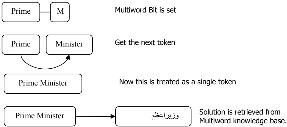
Fig. 1 Multiword recognition and Handling
