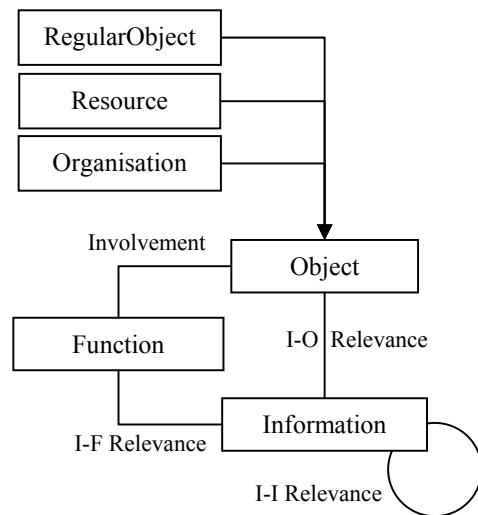
Fig. 3 The PARADIGMA Core Ontology
