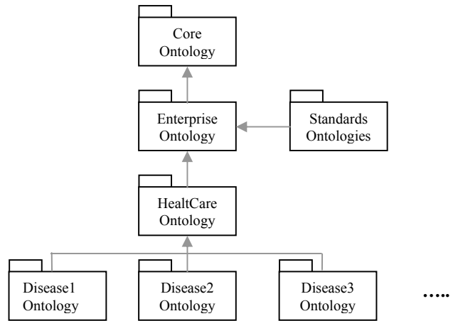
Fig. 2 Paradigma Reference Ontology Levels
