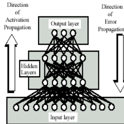
Fig. 2 Multilayer Perception
