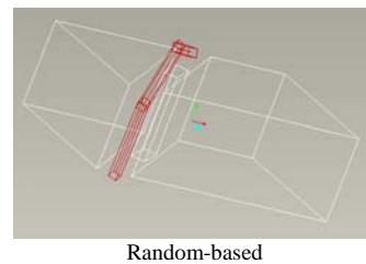
Fig. 9 Model 5: Diagonal empty space \{X^{\min} = -50, X^{\max} = 350, Y^{\min} = -50, Y^{\max} = 150, Z^{\min} = -200, Z^{\max} = 50; S = (25, 0, 0); T = (180, 100, -185); \text{Radius} = 5; N^{\text{turns}} = 100\}
