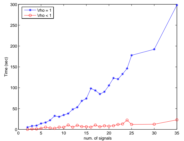
Fig. 2 Simulation times (in seconds) of FastICA
