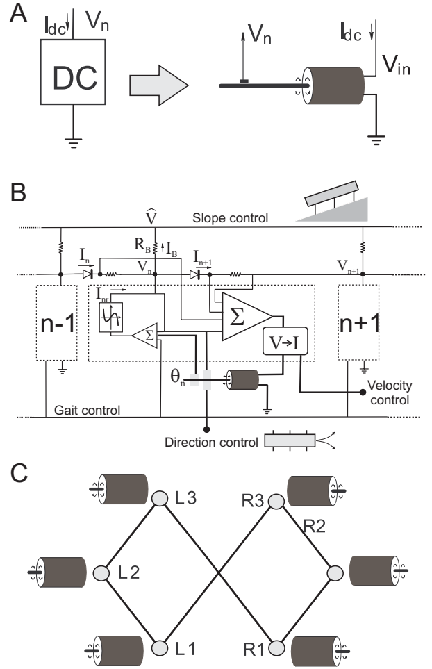
Fig. 6. CPG with the dynamics of the limb actuators integrated into the gait control. A) Scheme showing the point of the circuit to get the values of the variables V_n and I_{dc} in the case of DC block and motor. B) Feedback loop through the robot environment allowing to tune the CPG according to the robot task. DC-block (Fig. 3) is substituted by the motor-leg-sensor block, voltage adder, and voltage to current converter. C) Ring configuration. Filled circles correspond to electrical circuits with the motor dynamics replacing the double capacitors in the circuit.
