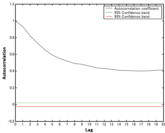
Fig. 2 Autocorrelation plot of the data series
