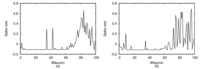
Fig. 9. (a) and (b) A example of the firing rate after firing (a) (\sigma_{sd}, \sigma_{cd}) = (1.0, 3.0) (b) (\sigma_{sd}, \sigma_{cd}) = (3.0, 1.0)
