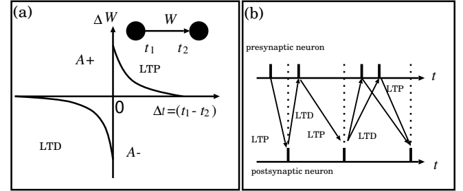
Fig. 2. (a) Window function of STDP.(b) Time Diagram shows that only spike pairs connected by arrows contribute to plasticity (near-neighbor interaction).
