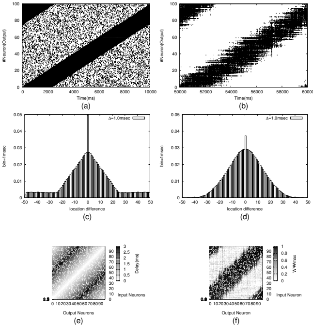
Fig. 4. Schematic illustration of self-organization. (a) The case that there is no inhibitory feedback inputs. (b) This model.
