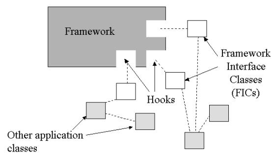
Fig. 1 Framework application classes
