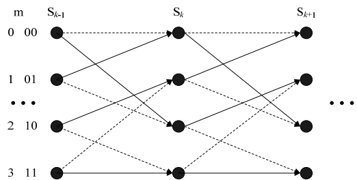
Fig. 4 Trellis diagram of the RSC code
