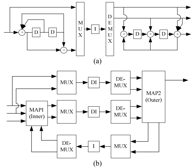
(a) Encoder (b) Decoder Fig. 3 Structure of Type III
