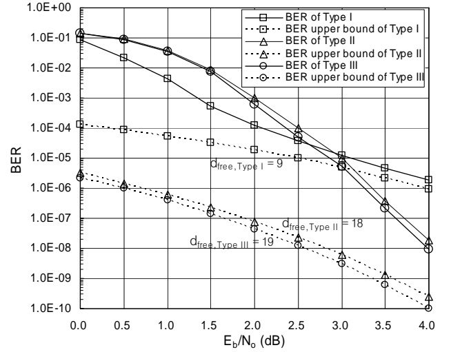
Fig. 8 BER and BER upper bound of the three types
