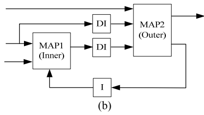
(a) Encoder (b) Decoder Fig. 1 Structure of Type I
