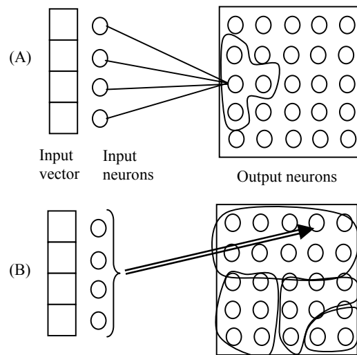
Figure 1 – Self-organizing Classification
