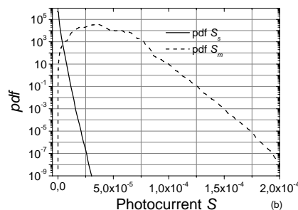
Fig. 5 Probability density function of the photocurrent at the receiver in the case of a) single span system with P_{in}=5\text{dBm} and b) multispan system with P_{in}=2\text{dBm}
