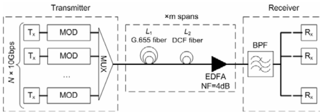
Fig. 1 System under investigation
