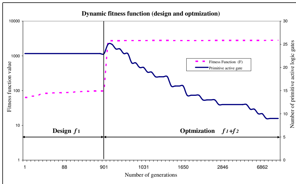
Fig. 8. This graphic shows the behaviour of the fitness function. Two different stages may be seen, design f1 and optimization ( f_1 + f_2 ). It is also notable that the number of primitive active gates is reduced.
