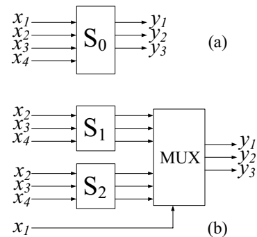
Fig. 14. Shannon decomposition.
