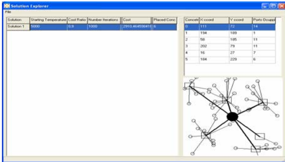
Fig. 5 Simulated Annealing solution for 1000 iterations on each temperature step
