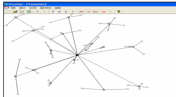
Fig. 8 Genetic Algorithm solution by the circumstances of step one from the experiments method
