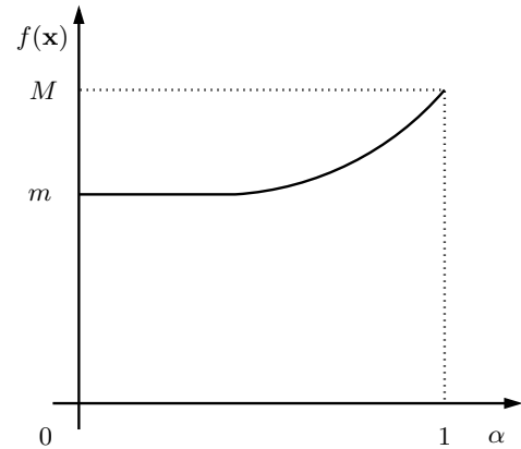
Fig. 5 Fuzzy solution
