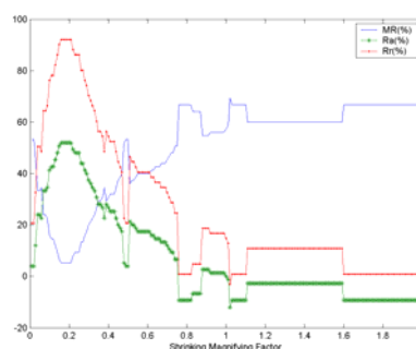
Fig. 1 Results of iris classification using RBFN
