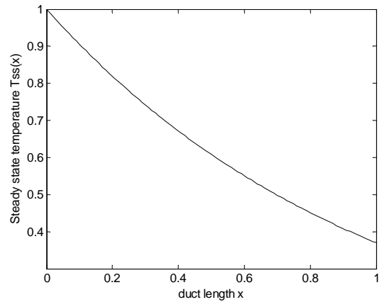
Fig. 3 Temperature steady state distribution for v=1
