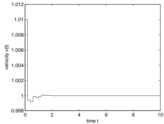
Fig. 9 Control moves, considering temperature at x = [0.2 \ 0.4 \ 0.6 \ 0.8 \ 1] as controlled variables
