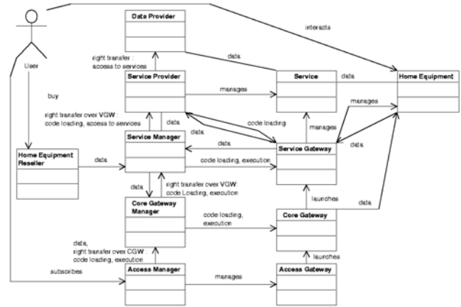
Fig. 3 RBac Model for Services at Home Delivery
