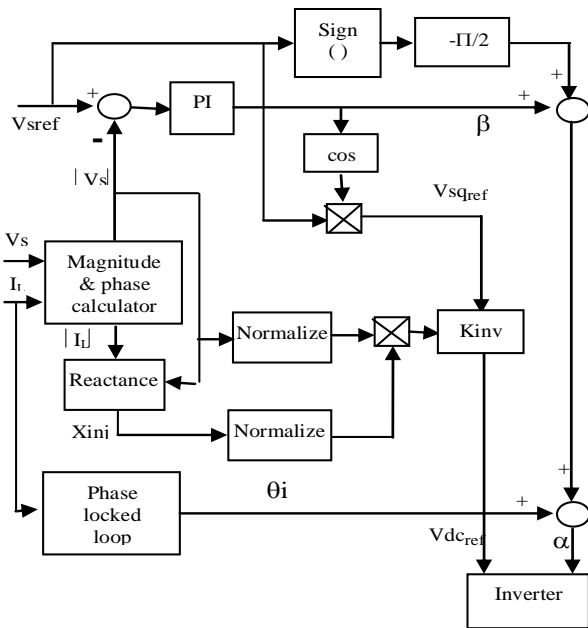
Fig. 9 Control block diagram of SSSC
