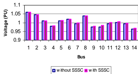
Fig. 4 The voltage profile of the IEEE 14 bus system for case 1
