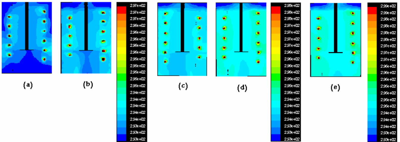
Fig. 4 Temperature contours in selected range for coiled tank by passage of time: (a) 1.2s, (b) 2.7s, (c) 4.8s, (d) 6.3s, (e) 7.8s. (Temperatures higher than the maximum value shown in temperature range bar are shown with the highest amount)
