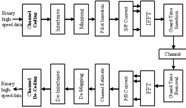
Fig. 4 Block diagram for multi-carrier transmission –OFDM
