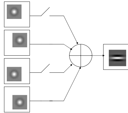
Fig. 7. Cascaded filter structure: For calculating the Gabor filter output at a particular position, selected DoG-filter outputs are added together.
