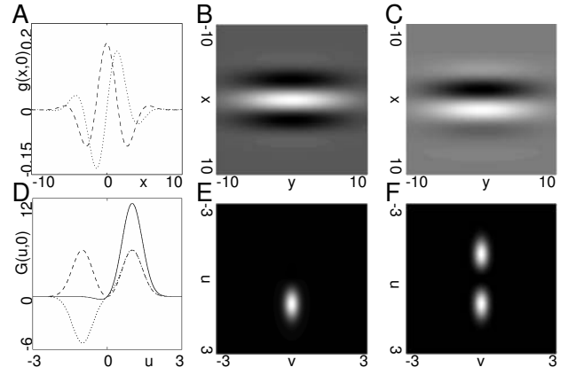
Fig. 2. Gabor function: A: shapes of real (dashed line) and imaginary(dotted line) part in x-direction. B,C: real and imaginary part as 2D profile. D: spectrum in u-direction(solid line), and spectra of real(dashed) and imaginary(dotted) part. E: 2D profile of the Gabor spectrum. F: 2D profile of the Fourier transformed real part.
