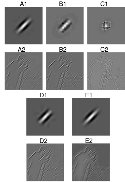
Fig. 4. Parameter variation: 1: synthesized filter masks, 2: results of test image filtering. A: \sigma_{1,0} = \frac{1}{\omega_0} , \Delta x_0 = \sigma_{1,0} . B: \sigma_{1,0} = \frac{1}{\omega_0} , \Delta x_0 = 2\sigma_{1,0} . C: \sigma_{1,0} = \frac{0.5}{\omega_0} , \Delta x_0 = 3\sigma_{1,0} . D: \sigma_{1,0} = \frac{2}{\omega_0} , \Delta x_0 = 0.5\sigma_{1,0} . E: \sigma_{1,0} = \frac{2}{\omega_0} , \Delta x_0 = \sigma_{1,0} . (Axes as in Fig. 3)
