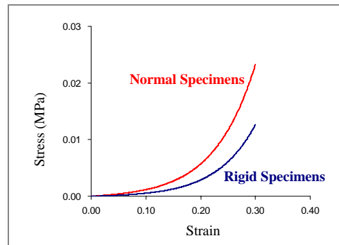
Fig. 4 Stress-Strain curves drawn from the hyperelastic material model determined from the compressive tests; the hyperelastic material model was used for presentation of non-linear mechanical characteristic of the specimens
