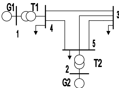
Fig. 2 Single line diagram of system 1
