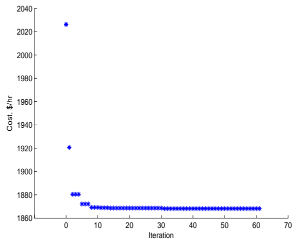
Fig. 3 Reduction cost function F
