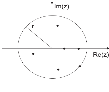
Fig. 1. Closed disk in the complex plane in which all zeros of a certain complex polynomial f \in \Pi_6 are situated.
