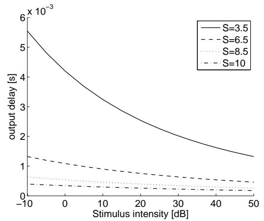
Fig. 3. Intensity-dependent output latency of 4 neurons with different transient sensitivity as a function of the stimulus intensity.
