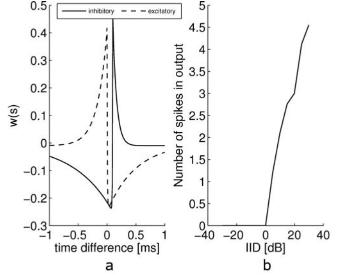
Fig. 4. a: Windows used for the STDP. b: Firing rate when neuron is presented with different IID's. Neuron taught with a stimulus of -15dB IID.
