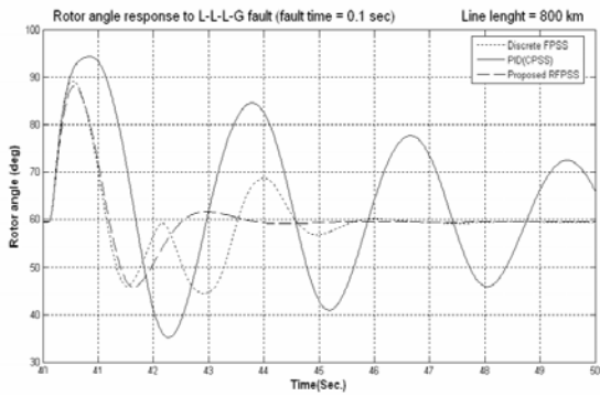
Fig. 10 (a) Fault duration = 0.10 sec.
