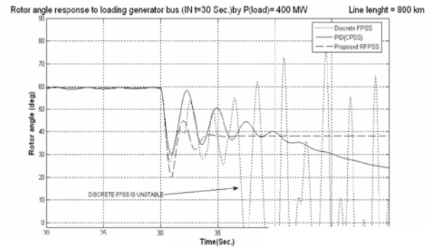
Fig. 11-d P(Load) = 400 MW
