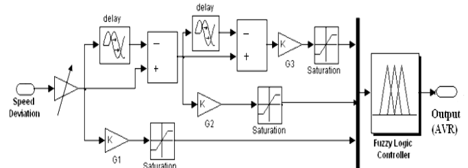
Fig. 6 block diagram of RFLPSS
