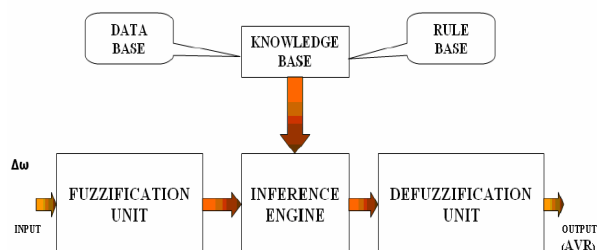
Fig. 3 Model of fuzzy controller and its blocks
