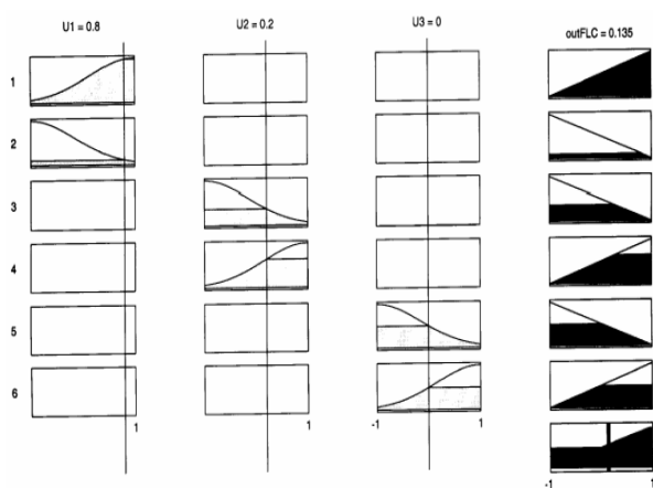
Fig. 7 Inference and defuzzification (Mamdani type)
