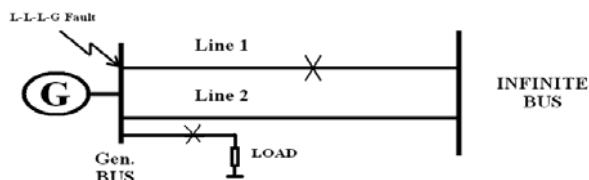
Fig. 2 Fault occurred on the bus of generator, line outage (line 1) and sudden load entrance
