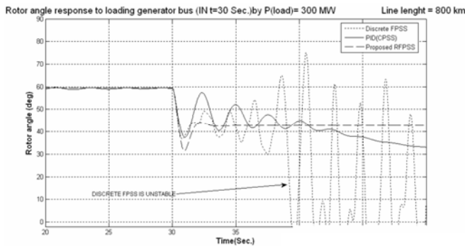
Fig. 11-c P(Load) = 300 MW
