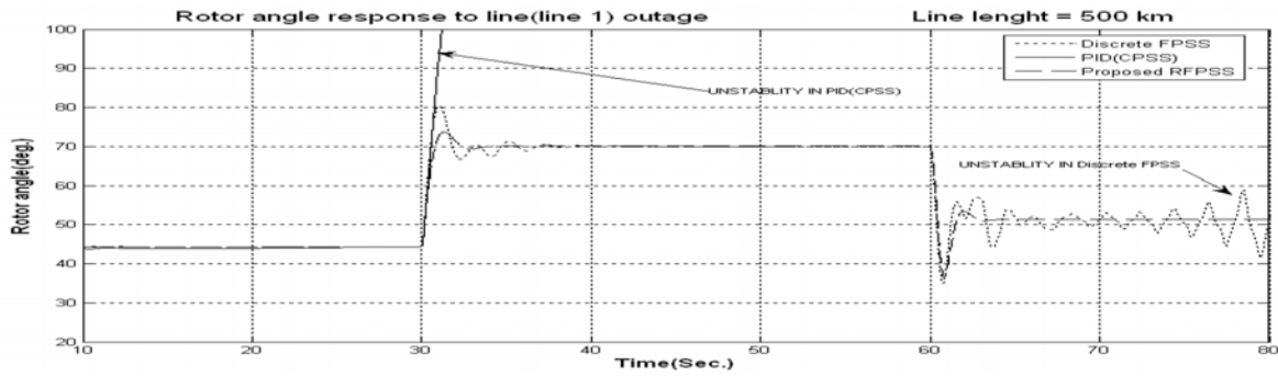
Fig. 9-b L=500 Km
