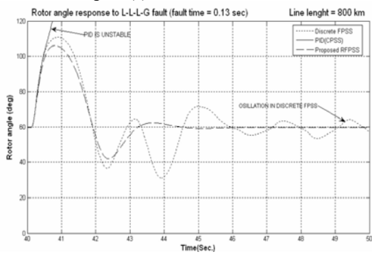
Fig. 10 (c) Fault duration = 0.13 sec.
