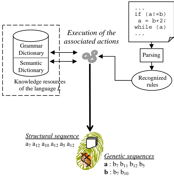
Fig. 2 Fingerprint extraction
