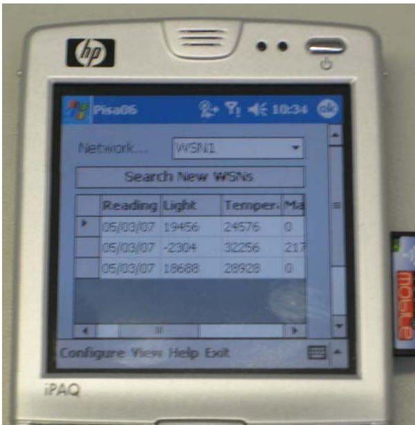
Fig. 5. Front-end application
