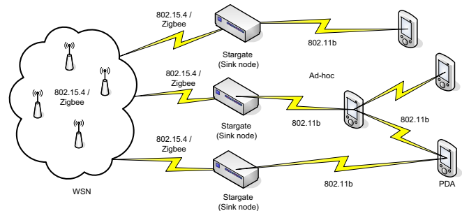
Fig. 4. Prototype layout
