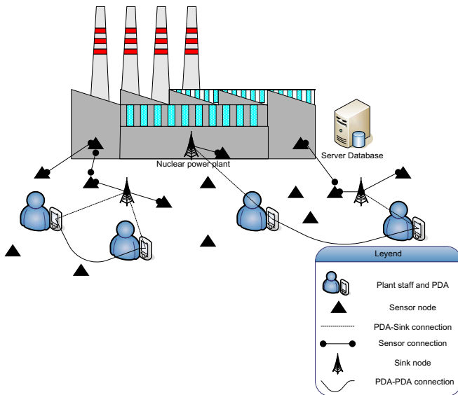
Fig. 1. Operational setting
