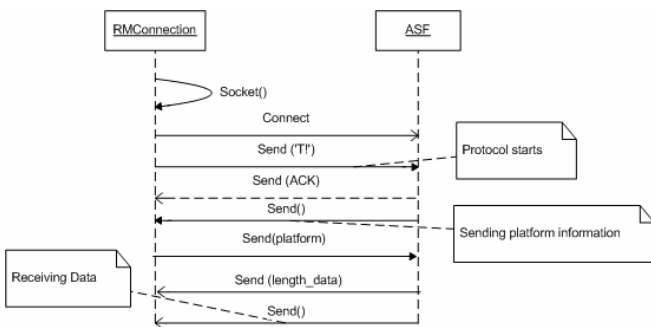
Fig. 6. SerialForwarder connection protocol
