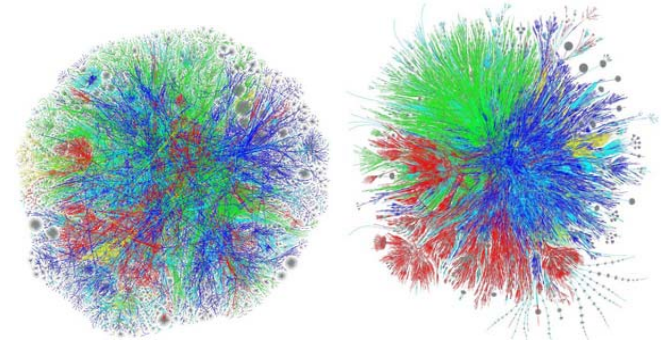
Fig. 7. Left and Right are the layout results of model D with the LGL method and FR-HI method, respectively. The color classification of the edges are according to the domain region as "Asia Pacific - Red", "Europe/Middle East/Central Asia/Africa - Green", "North America - Blue", "Latin American and Caribbean - Yellow", "RFC1918 IP Addresses - Cyan", and "Unknown - gray".
