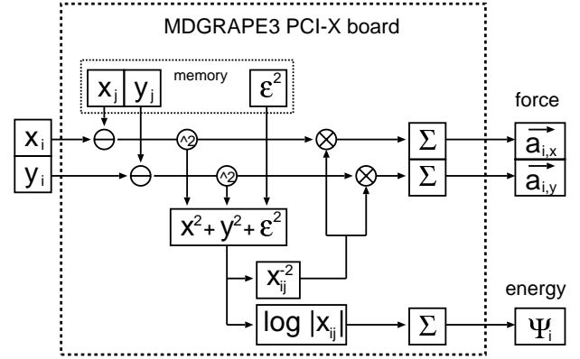
Fig. 3. The pipeline image of the architecture of MDGRAPE-3.
