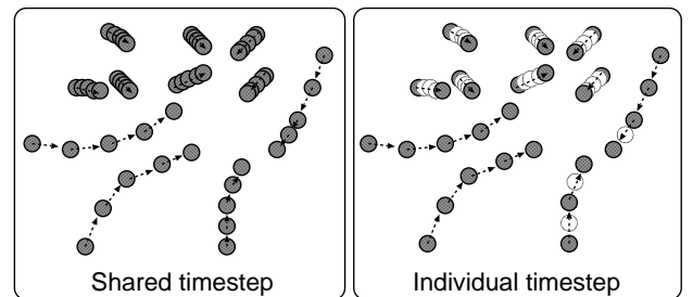
Fig. 1. The left and right figures show a the schematic figure of time evolution for the shared and individual timestep scheme, respectively. For Individual timestep, longer timestep nodes are calculated as predictor \odot .
