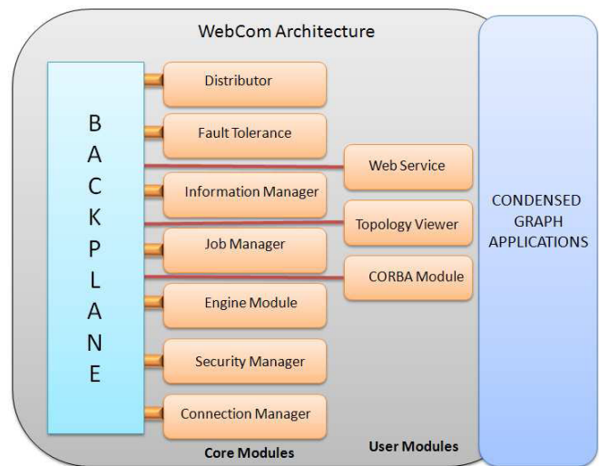
Fig. 1 WebCom architecture
