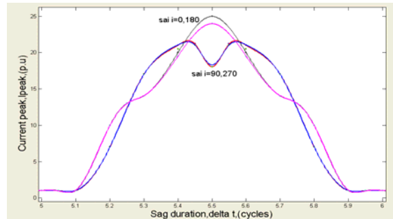
Fig. 6 Maximum inrush current versus different voltage sag duration in voltage sag type A with h=0.4
