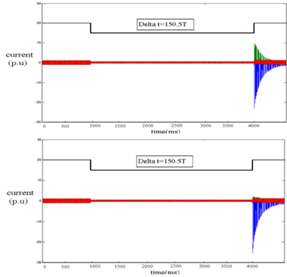
Fig. 5 (a) Three leg and (b) Five leg Transformer current for a sag type v(h=0.4, \Delta t=150.5T, \psi_i=0)
